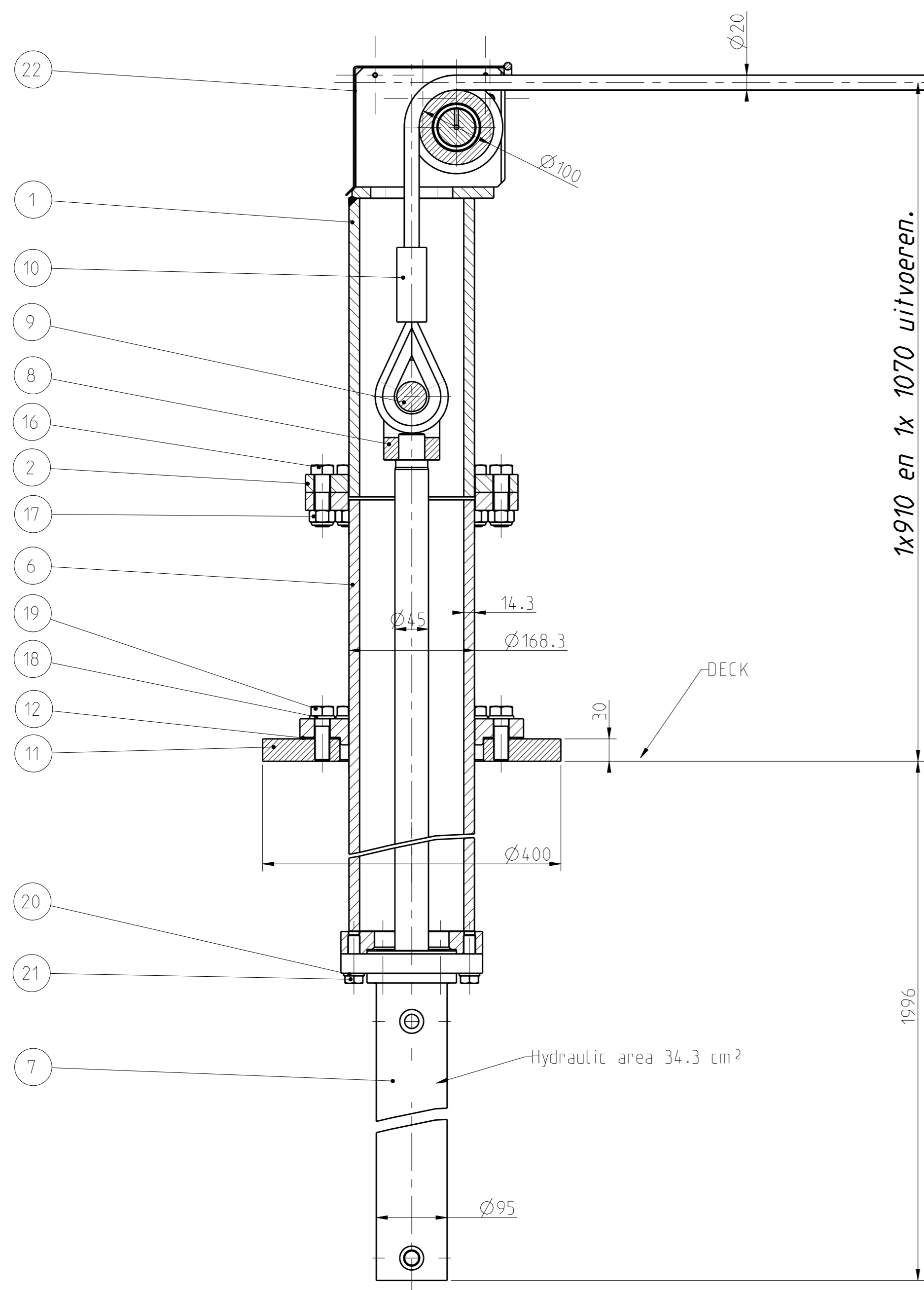
SECTION X-X
